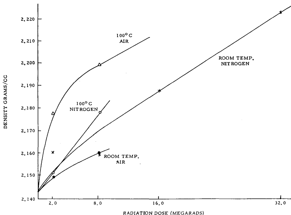
Fig. 1. Density changes in Teflon irradiated under different environmental conditions.
