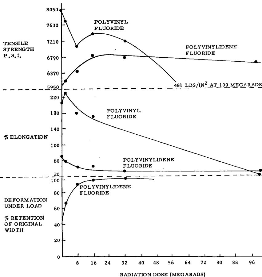
Fig. 2. Physical changes in irradiated polyvinyl fluoride and polyvinylidene fluoride.
